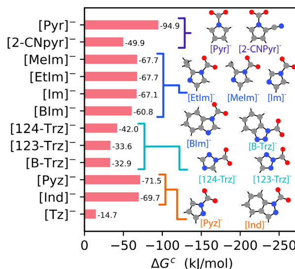
Fig. 4 The [HBAAa] - CO 2 complexation free energies (in kJ mol -1 ), where \Delta G^c = \Delta G_2 . The figure is organized by structural similarity to compare how functionalization impacts CO 2 binding. Chemical structures are included to illustrate structural similarities and differences. Atom color key: gray = carbon, blue = nitrogen, red = oxygen, white = hydrogen. Different families of [HBAAa] - species are denoted with the purple, blue, teal, and orange brackets.
