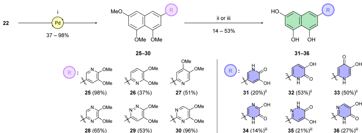
Scheme 4 Reagents and reaction conditions: (i) heteroarylhalide (39/40/41/43/44/45), Pd(PPh 3 ) 4 (10 mol%), K 2 CO 3 , 1,4-dioxane/H 2 O (3:1), 100 °C, 16 h; (ii) BBr 3 , DCM, 0 °C → r.t., 48 h; (iii) (a) BBr 3 , DCM, 0 °C → r.t., 6–24 h; (b) 4 M HCl (1,4-dioxane), 1,4-dioxane, 110 °C, 16 h, 5–24 h.
