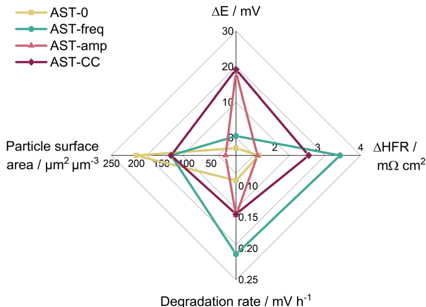
Fig. 6 Spider plot to visualize performance losses ( \Delta E and \Delta HFR ) and possible long-term degradation (degradation rate and particle surface area in the membrane) with the four stress tests. Note that for all parameters, a high value means more degradation or worse performance. The degradation rates shown are from the linear trend analysis.
