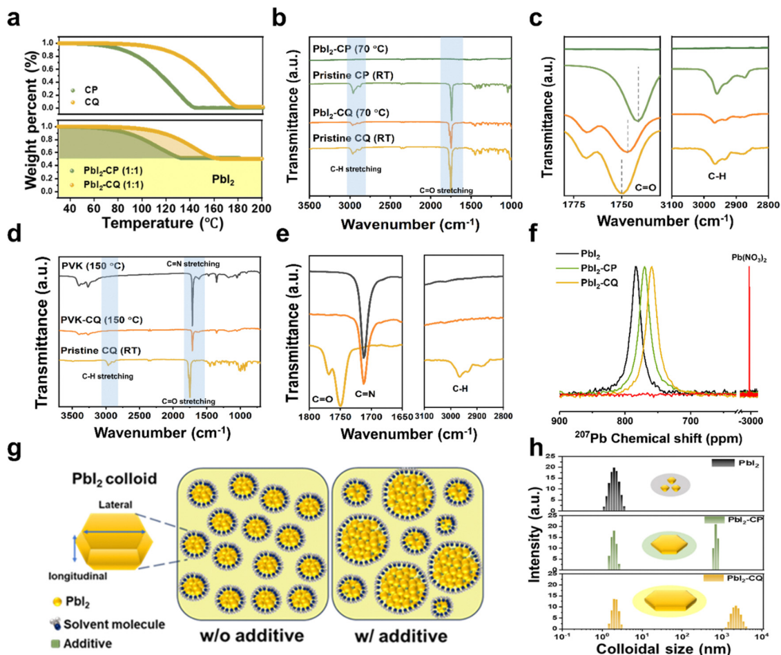
Fig. 2 Volatility and interaction of CP and CQ additives. (a) TGA plots of CP and CQ (pristine and blended with \text{PbI}_2 ). (b) The whole range and (c) magnified FTIR spectra of CP (RT), CQ (RT), \text{PbI}_2 -CP (70 °C), and \text{PbI}_2 -CQ (70 °C). (d) The whole range and (e) magnified FTIR spectra of CQ, PVK-CQ (150 °C), and PVK without CQ (150 °C). (f) ^{207}\text{Pb} NMR spectra of \text{PbI}_2 , \text{PbI}_2 -CP, and \text{PbI}_2 -CQ, where the samples were calibrated by \text{Pb}(\text{NO}_3)_2 , which represents -2959.7 ppm. (g) Schematic diagram of the \text{PbI}_2 colloids (with or without additive). (h) DLS measurements of pristine \text{PbI}_2 , \text{PbI}_2 -CP, and \text{PbI}_2 -CQ. The inset shows the schematic diagram of the evolution of \text{PbI}_2 flakelets.
