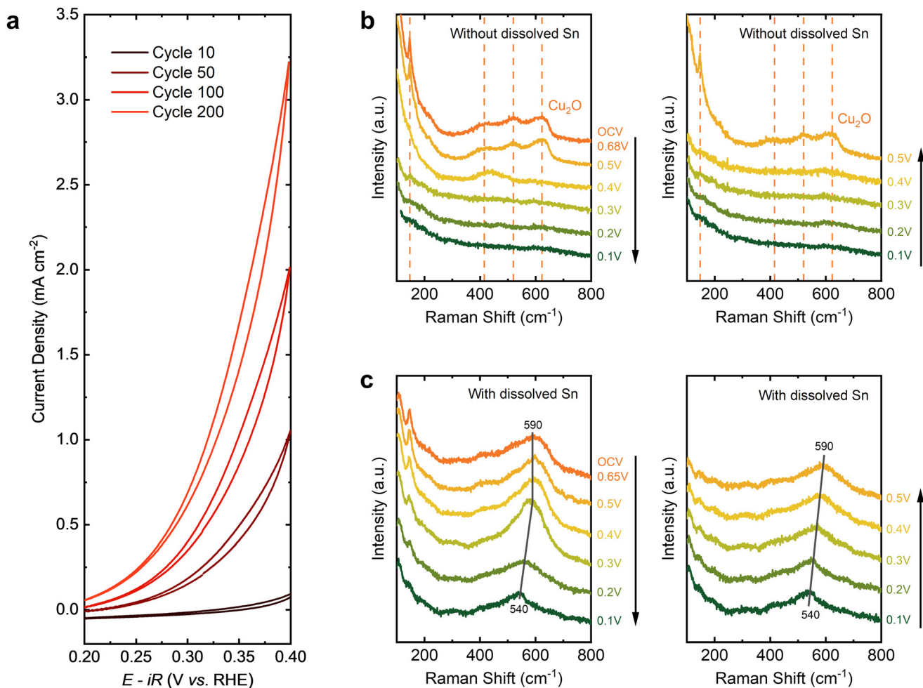
Fig. 4 (a) Cyclic voltammety on Cu disk in Ar-saturated 1 M KOH + 50 mM \text{Sn}(\text{OH})_3^- at 10 \text{ mV s}^{-1} and 800 rpm. (b) In situ EC-Raman spectra on Cu nanoparticle electrode in Ar-saturated 4 M KOH. (Left) Polarization in the cathodic direction from pristine electrode. (Right) Subsequent polarization in the anodic direction. (c) In situ EC-Raman spectra on Cu nanoparticle electrode in Ar-saturated 4 M KOH and 0.1 M \text{Sn}(\text{OH})_3^- (prepared with 4.1 M KOH and 0.1 M SnO). (Left) Polarization in the cathodic direction from pristine electrode. (Right) Subsequent polarization in the anodic direction. The electrode is scanned and held at each potential (vs. RHE) for at least 2 min before taking Raman measurements. Orange dashed lines: \text{Cu}_2\text{O} reference bands. 43,44 Gray solid lines: band assigned to surface \text{Sn}(\text{OH})_x (guides to the eye).
