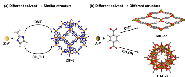
Fig. 7 Solvent selection influence on the structures of MOFs under similar conditions. Atom code: C, grey; O, red; H, white; Zn, yellow; Al, dark yellow.
