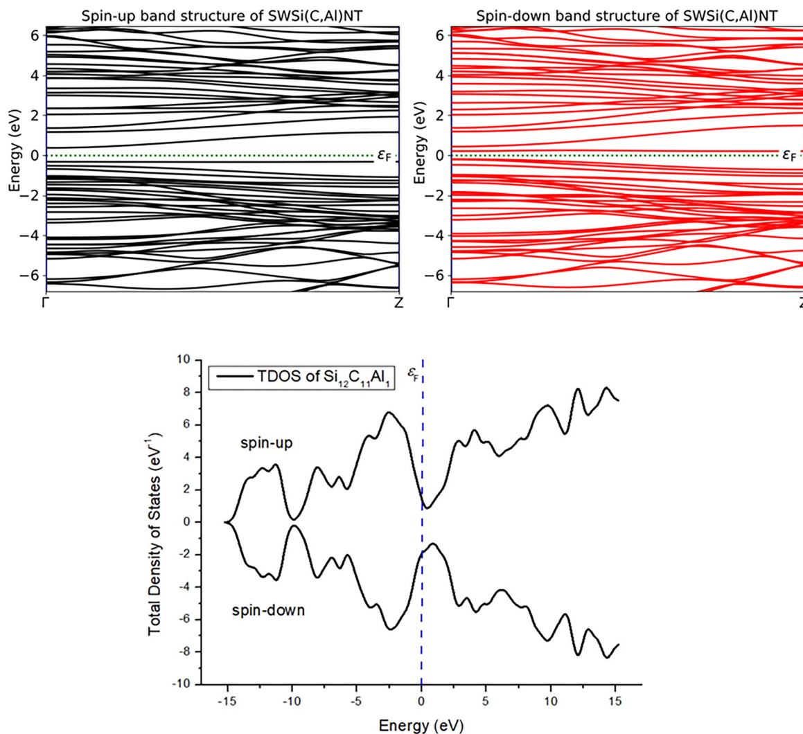
Fig. 7 Spin-up (black) and spin-down (red) band structures of \text{Si}_{1-x}\text{C}_x\text{Al}_x NT, along with the TDOS. A spin asymmetry in the band gap is evident.
