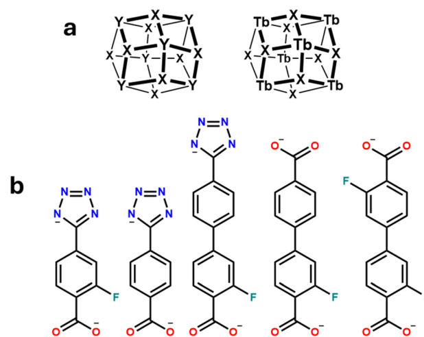
Fig. 2 (a) Clusters and (b) linkers used by Eddaoudi et al. to obtain RE(III) fcū MOFs.
