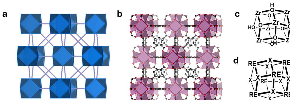
Fig. 1 (a) fcū net, (b) structure of UiO-66, (c) [Zr_6O_4OH_4]^{12+} cluster of Zr-UiO-66, and (d) [RE_6X_8]^{10+} cluster of RE-UiO-66, where X = OH or F.
