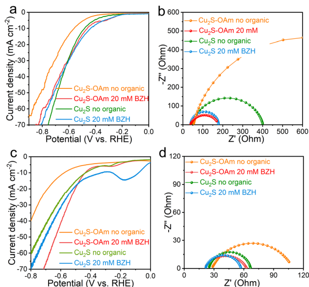
Fig. 3 (a) LSV curves and (b) Nyquist plots at -0.7 V vs. RHE of Cu 2 S-OAm and Cu 2 S in 1 M sodium acetate-acetic acid electrolyte (pH = 5.2) with and without BZH at room temperature; (c) LSV curves and (d) Nyquist plot at -0.7 V vs. RHE of Cu 2 S-OAm and Cu 2 S in 1 M potassium carbonate-potassium bicarbonate electrolyte (pH = 9) with or without BZH at room temperature.
