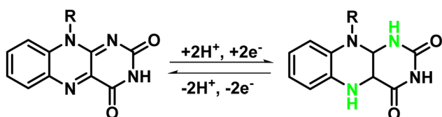
Scheme 2 Faradaic reaction of flavin units in PEO-KOH gel solution.
