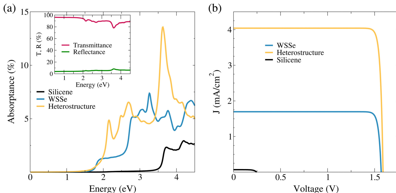
Fig. 4 (a) Optical absorbance of monolayer WSe 2 (blue), silicene (black), and the WSe 2 /Si interface (yellow). (b) Current density as a function of voltage for the three studied systems. The inset shows the transmittance (red) and reflectance (green) of the WSe 2 /Si interface.
