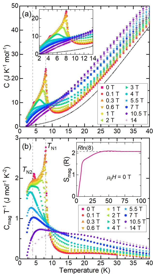
Figure 5. Heat capacity of \text{EuHfSe}_3 . (a) Molar heat capacity ( C_p ) at several applied fields; the dashed line indicates the background ( C_{bg} ) for the \mu_0H = 0 T curve extrapolated to T = 0 K; see methods and Fig. S11 for details. The inset shows the low-temperature region. (b) Heat capacity related to the low-temperature peaks ( C_{mag} ) calculated by subtracting C_{bg} from the molar C_p . The inset shows the entropy of the low-temperature peaks ( S_{mag} ) normalized per formula unit for the \mu_0H = 0 T curve. The vertical dashed lines denote the transition temperatures.
