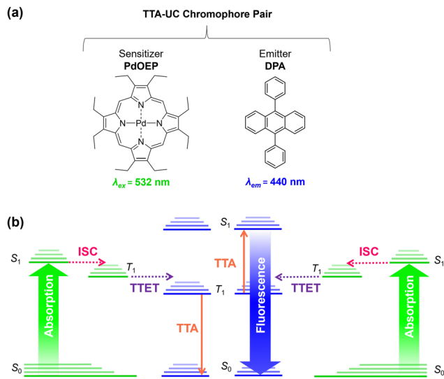
Fig. 1 Triplet-triplet annihilation upconversion is a multi-step photophysical process between two chromophores. (a) Structures of the benchmark chromophore pair used in this study: PdOEP (sensitizer) and DPA (emitter). (b) Mechanism of TTA-UC. (i) The absorption of photons by the sensitizer PdOEP (green arrow) results in formation of the excited singlet state ( S_1 ), which relaxes by intersystem crossing (ISC, pink dashed arrow) to the excited triplet state ( T_1 ). (ii) Triplet sensitizers then collide with emitters to produce triplet emitters via triplet-triplet energy transfer (TTET, purple dashed arrow) if their energy levels overlap within the Dexter radius. (iii) Triplet emitters then collide with each other, leading to triplet-triplet annihilation (orange dashed arrow), whereby one molecule is excited to a higher energy level, and the second relaxes to the ground state. Radiative relaxation of the higher energy state leads to photon emission via fluorescence (blue arrow).
