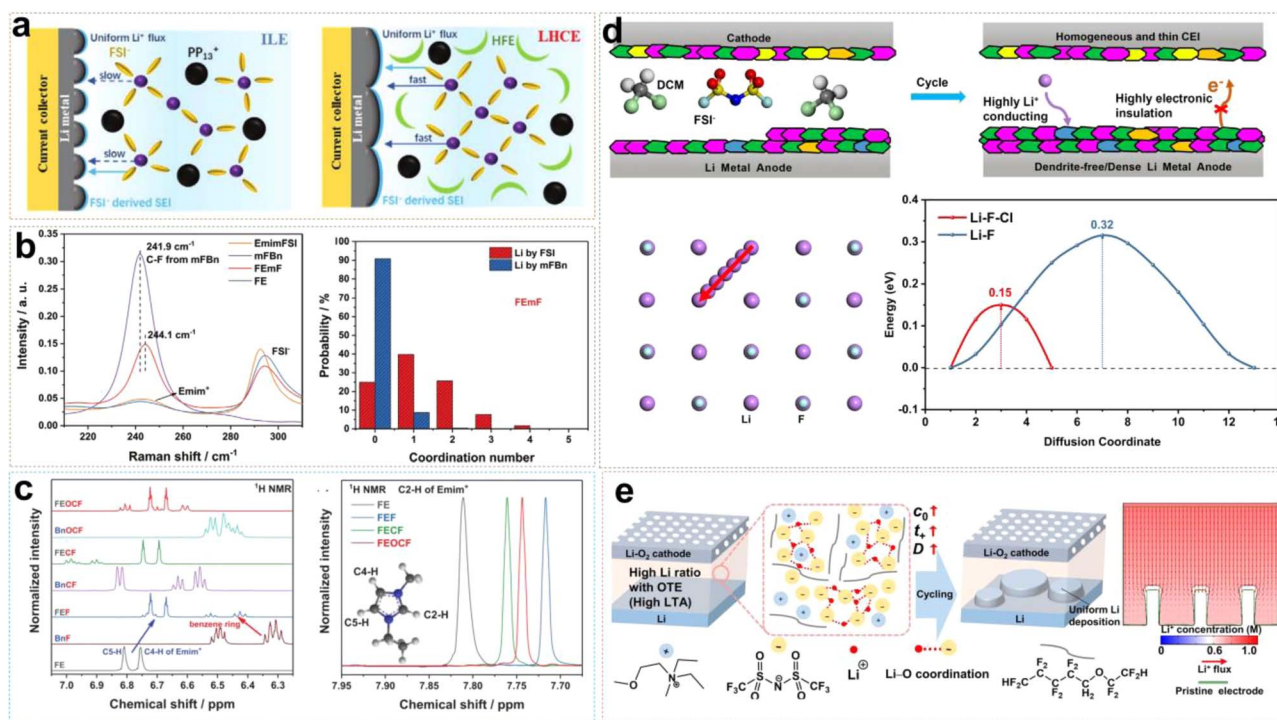
Fig. 8 (a) Schematic diagrams of Li plating on a Cu current collector and solvation structures of ILE and LHCE. Reprinted from ref. 51 with permission. Copyright 2021, Wiley. (b) \text{Li}^+ ion solvation structure with mFBn and the corresponding Raman characterization and coordination number calculation. Reprinted from ref. 52 with permission. Copyright 2022, Wiley. (c) 1D ^1\text{H} NMR spectra of the electrolytes and their constituents in the region of 6.25–7.05 ppm and 7.675–7.950 ppm. Reprinted from ref. 53 with permission. Copyright 2023, Wiley. (d) Schematic illustrations of the SEI/CEI components from LCM systems and \text{Li}^+ diffusion path and migration energy barriers of \text{Li}^+ along LiF–LiCl grain boundaries. Reprinted from ref. 54 with permission. Copyright 2024, American Chemical Society. (e) Schematic diagram of Li deposition behavior by regulating T_{\text{sand}} with OTE. Reprinted from ref. 55 with permission. Copyright 2021, Wiley.
