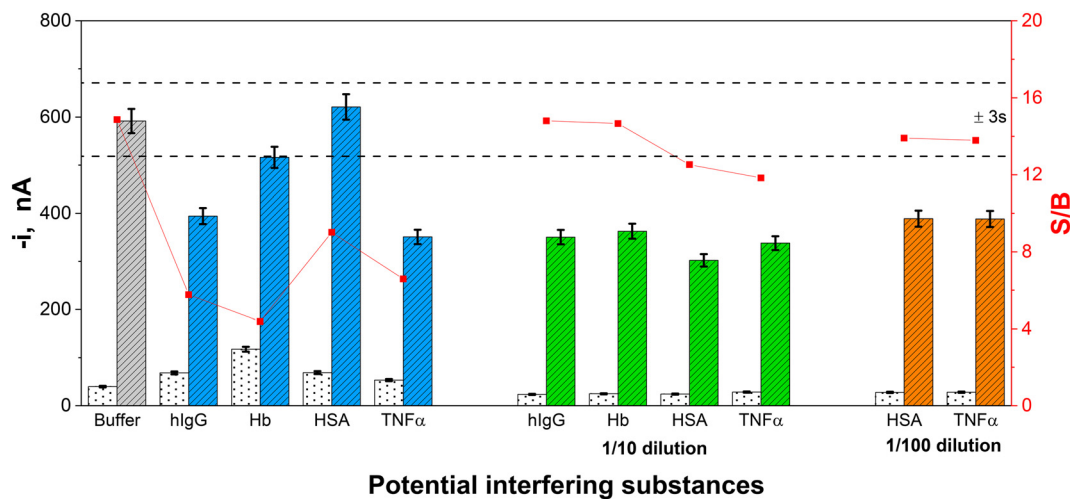
Fig. 3 Amperometric responses provided by the developed bioplatfor for 0 (dotted bars) and 2500 \text{pg mL}^{-1} GDF-15 (striped bars) standards prepared in the absence and in the presence of 1 or 0.1 \text{mg mL}^{-1} hIgG, 5 or 0.5 \text{mg mL}^{-1} Hb, 50, 5.0 or 0.5 \text{mg mL}^{-1} HSA and 10, 1.0 or 0.1 \text{ng mL}^{-1} TNF \alpha . S/B ratio values were displayed using red dots, whereas control limits (dashed black lines) were set at three times the standard deviation of the S/B mean value of three measurements obtained in the absence of interferent.
