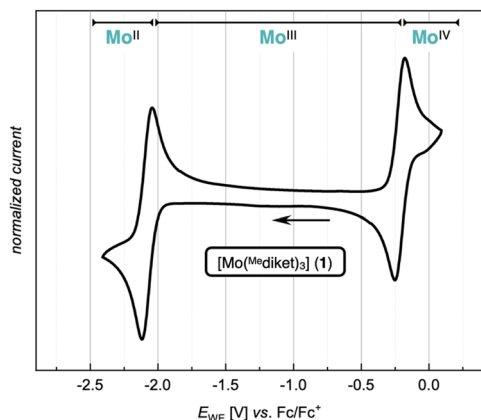
Fig. 2 CV of [\text{Mo}^{\text{Me'diket}}_3] ( 1 ) (1 mM) in TBAPF 6 /MeCN (0.1 M) at a scan rate of \nu = 100 \text{ mV s}^{-1} .
