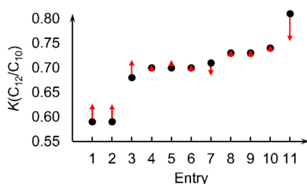
Fig. 6 Experimental K(C_{12}/C_{10}) values of complex I ( L_1 = \text{Me} ) (black dots) vary between 0.59 and 0.81 under different reaction conditions (Table 2). 14 Red arrows indicate differences between the experimental K -values and the predicted K -values from a model utilizing the 6 physical and 8 molecular features.
