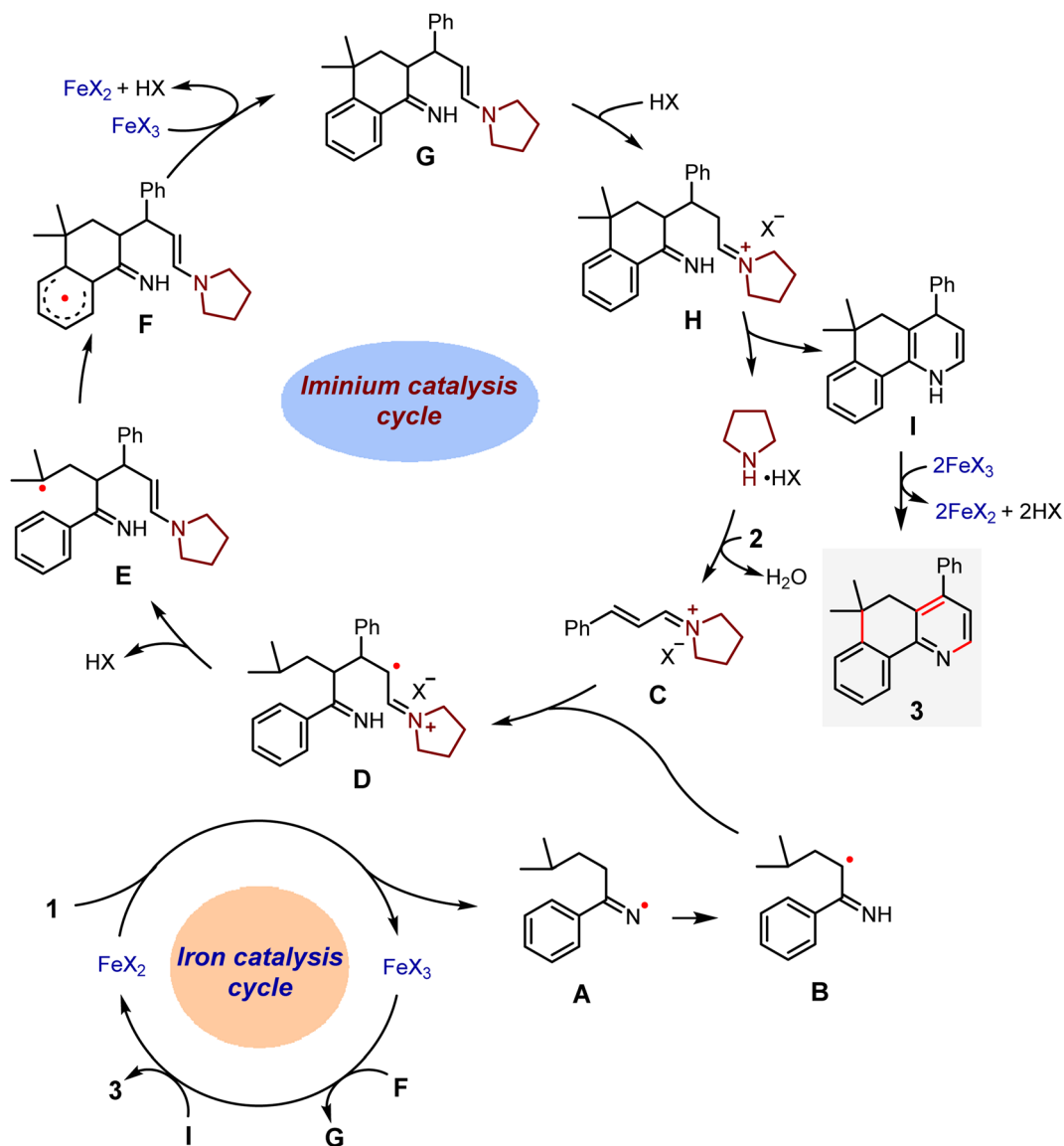
Scheme 7 Proposed mechanism for the relay annulation via synergistic iron and iminium catalysis ( \text{X} = \text{ClO}_4 , OBz, or acac).
