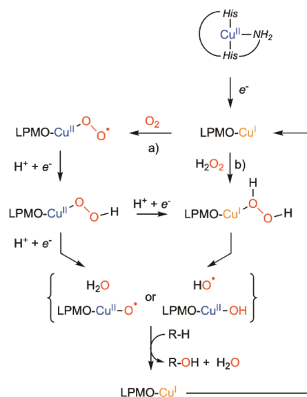
Scheme 3 Putative mechanisms to explain LPMO catalyzed hydroxylation: (a) the monoxygenase pathway and (b) peroxxygenase pathway.
