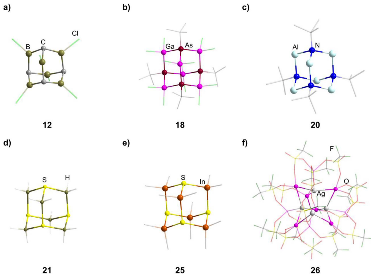
Fig. 2 Examples of adamantane-type compounds with group 13 atoms in the E position: [(CH)_4(BCl)_6] ( 12 , top left (a)), [Li(thf)_4]_2[Li(BuAs)_4(GaCl_2)_6] ( 18 , top center (b)), Li_2[Li(BuN)_4(AlH_2)_6] ( 20 , top right (c)), Na_2[S_4(BH_2)_6] ( 21 , bottom left (d)), DMPyr_2[S_4(InMe_2)_6] ( 25 , bottom center (e)) and [Ga(C_6H_5Me)_2]_2[AgGa(OTf)_3]_4Ga_6(OTf)_4 ( 26 , bottom right (f)). Hydrogen atoms in the organic ligands and counterions, if present, are omitted for clarity.
