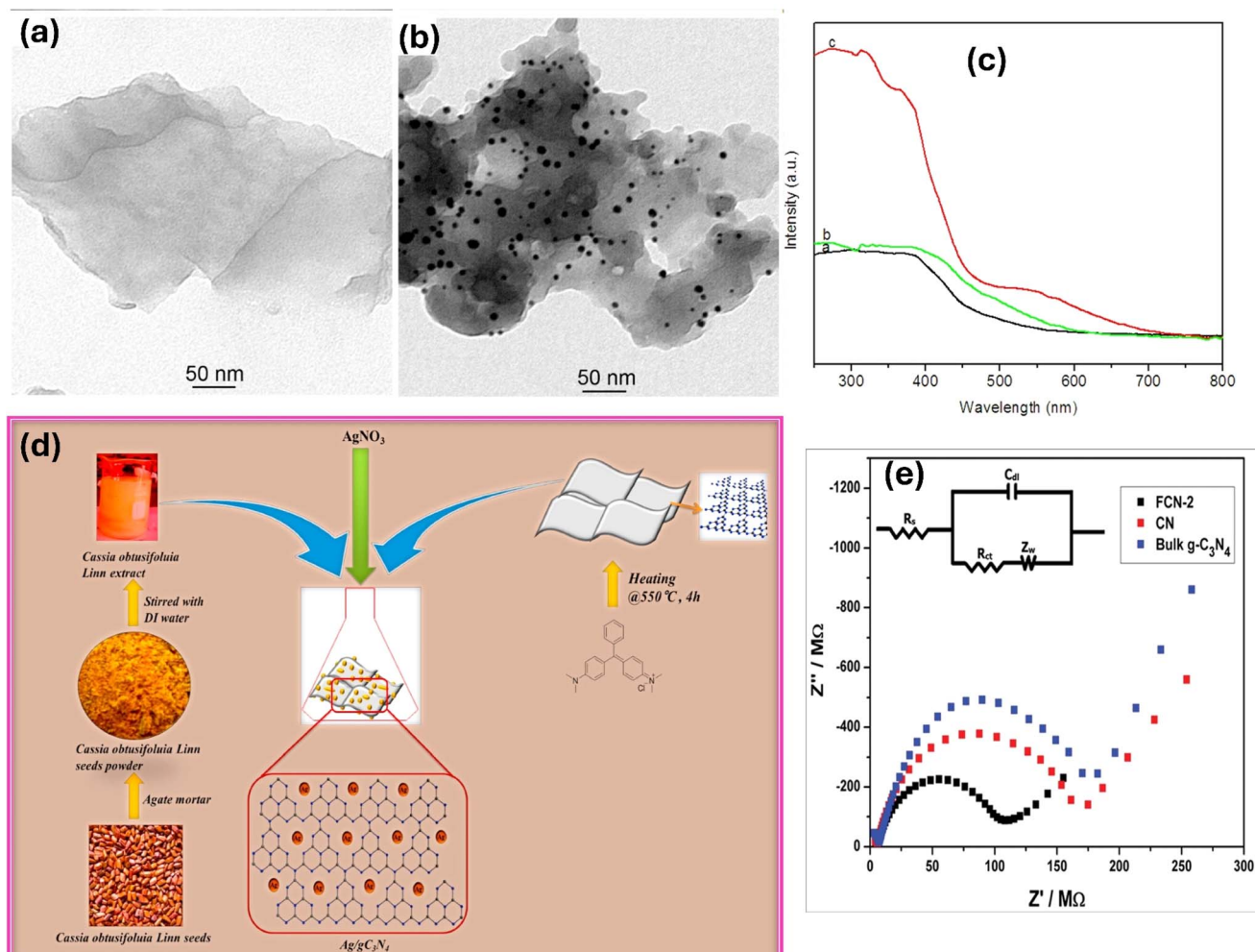
Fig. 2 Tem image of (a) \text{g-C}_3\text{N}_4 , (b) \text{Au/g-C}_3\text{N}_4 , (c) DRS data of \text{g-C}_3\text{N}_4 nanosheets, bulk \text{g-C}_3\text{N}_4 , and \text{AuNP/g-C}_3\text{N}_4 nano hybrids reprinted with the permission of ref. 72, copyright 2024, American Chemical Society; (d) synthesis of \text{Ag/g-C}_3\text{N}_4 via green route, reprinted with the permission of ref. 73, copyright 2024, Elsevier; and (e) EIS of the \text{g-C}_3\text{N}_4 , and pure and Fe-doped \text{g-C}_3\text{N}_4 nanosheets, reprinted with the permission of ref. 74, copyright 2024, RSC.
