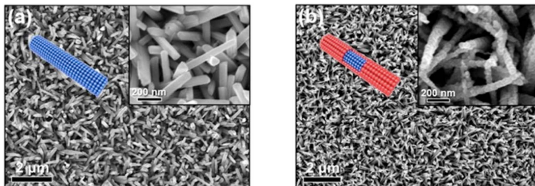
Fig. 14 (a) SEM images of Te NWs before and (b) after the detection of 1 \mu\text{M} Hg(II) ions (reproduced from ref. 118, with permission from Elsevier Ltd, Copyright © 2019).
