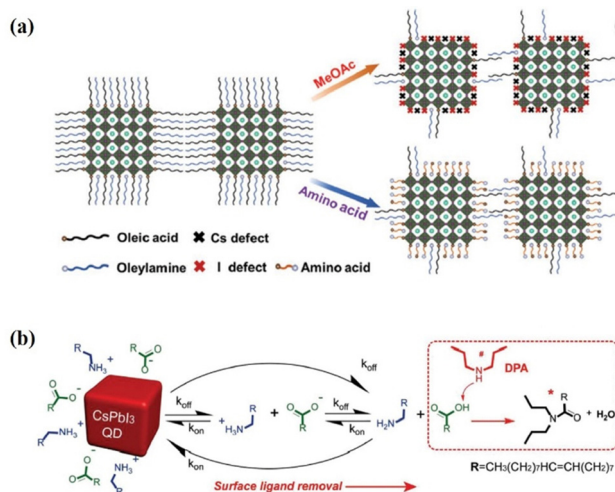
Fig. 14 (a) Schematic illustration of the changes on the PCD surface with conventional MeOAc rinsing and dual-passivation ligands before and after ligand exchange. Reproduced with permission from ref. 141. Copyright 2020, Wiley-VCH. (b) Schematic representation of the PCD dynamic surface stabilization and the ligand removal process assisted by DPA. Reproduced with permission from ref. 142. Copyright 2020, Wiley-VCH.
