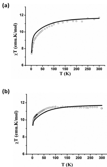
Fig. 3 Experimental (symbols) and predicted (solid line) temperature-dependence of \chi_M T from 2 to 300 K, at 0.1 T of 2a_des (a) and 2b (b). We have added a TIP value of 0.005 \text{emu mol}^{-1} to correct the experimental \chi T value of 2a_des . We have added a scaling factor of 0.9 to correct the experimental \chi T value of 2b . A dipolar coupling ( z_j ) of -0.05 and -0.01 \text{ cm}^{-1} was considered in our calculations for 2a_des and 2b , respectively, to simulate the experimental magnetic data.
