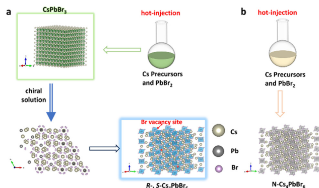
Fig. 1 (a) Schematic of the phase transformation from 3D cubic CsPbBr 3 to hexagonal 0D R - and S -Cs 4 PbBr 6 NCs. (b) Schematic of the synthesis of N-Cs 4 PbBr 6 NCs.
