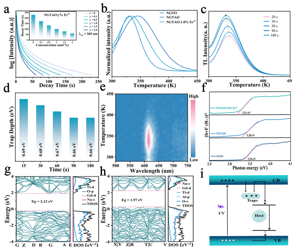
Fig. 5 (a) Afterglow decay curves of NGTAO: y\%\text{Er}^{3+} ( 0.1 \leq y \leq 2.0 ) after 365 nm UV irradiation. (b) TSL curve of the NGTO, NGTAO, and NGTAO:1.0% \text{Er}^{3+} phosphors after 365 nm excitation for 5 minutes. (c) TSL curve of the NGTAO:1.0% \text{Er}^{3+} phosphor at different time intervals after 5 minutes of excitation under 365 nm UV. (d) Trap depth distribution in NGTAO:1.0% \text{Er}^{3+} . (e) Contour plot of the TL curve of the NGTAO:1.0% \text{Er}^{3+} after 365 nm illumination. (f) The band gap values of NGTO, NGTAO, and NGTAO:1.0% \text{Er}^{3+} . Calculated electronic band structures and DOS of (g) NGTO and (h) NGTAO. (i) An energy diagram with a proposed plausible mechanism for the afterglow and PL mechanism.
