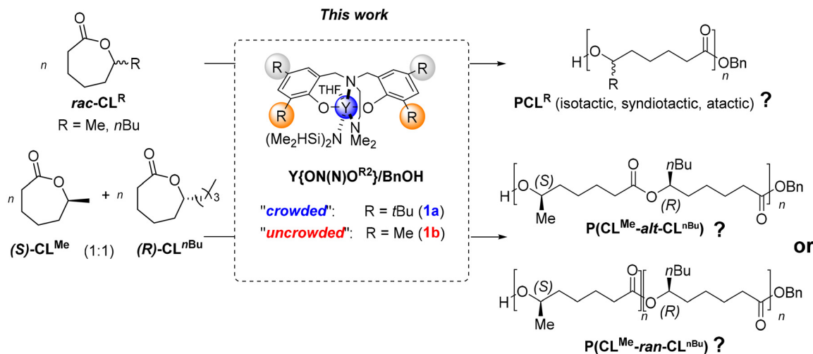
Scheme 3 ROP of 1-substituted- \epsilon -caprolactones ( rac\text{-CL}^R ; R = Me, n Bu) and ROCOP of equimolar mixtures of opposite-configuration, enantiopure monomers studied in the present work to assess the stereoselectivity ability of discrete yttrium complexes towards such seven-membered lactones.
