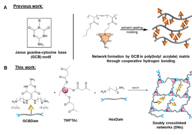
Scheme 1 (A) Previous strategy of Janus guanine–cytosine base (GCB) motifs being employed to prepare dissociative dynamic networks. (B) Current strategy of GCB motifs being employed to supplement associative vinylogous urethane.
