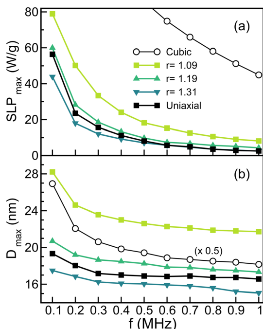
Fig. 8 Frequency dependence of the (a) maximum SLP and (b) the corresponding particle size extracted from the curves in Fig. 7 for different nanoparticle elongation ratios r = 1.09, 1.19, and 1.31 (colored symbols) and also for the cases of only uniaxial (black squares) or only cubic contribution (empty circles) with K_{u,c} = 1.1 \times 10^4 J m ^{-3} . Notice that D_{\max} for the last case has been rescaled by 0.5.
