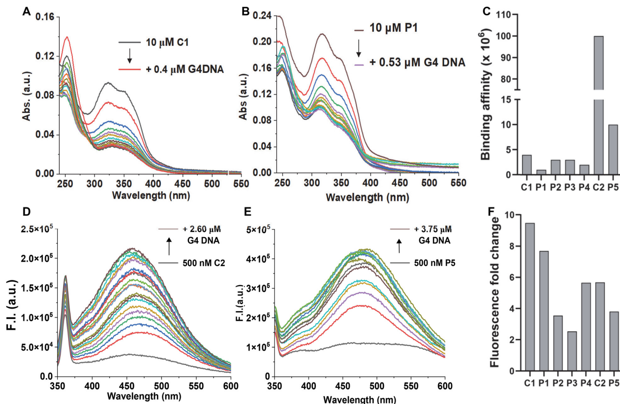
Fig. 5 UV-Vis titration spectra of 10 μM ligands (A) C1 and (B) P1, and (C) binding affinities for all the molecules in 10 mM Tris-HCl (pH 7.4), 0.1 mM EDTA and 0.1 M KCl with 10 μM pre-formed Hum 21-mer G4 DNA. Fluorescence titration spectra of 0.5 μM ligands (D) C2 and (E) P5, and (F) fold-change for all the molecules in 10 mM Tris-HCl (pH 7.4), 0.1 mM EDTA and 0.1 M KCl with 10 μM pre-formed Hum 21-mer G4 DNA.
