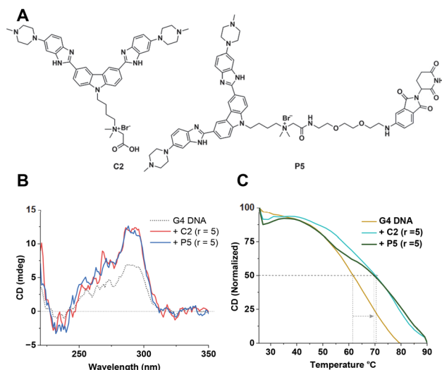
Fig. 4 (A) Chemical structures of molecules C2 and P5. (B) CD spectra of 3 μM Hum 21-mer G4 DNA alone, and with compounds C2 and P5 (15 μM) in 10 mM Tris-HCl (pH 7.4) containing 0.1 M KCl and 0.1 mM EDTA. (C) CD melting profiles of the pre-formed Hum 21-mer G4 DNA alone, and G-quadruplex DNA incubated with ligands C2 and P5 (15 μM) in 10 mM Tris-HCl (pH 7.4) containing 0.1 M KCl and 0.1 mM EDTA.
