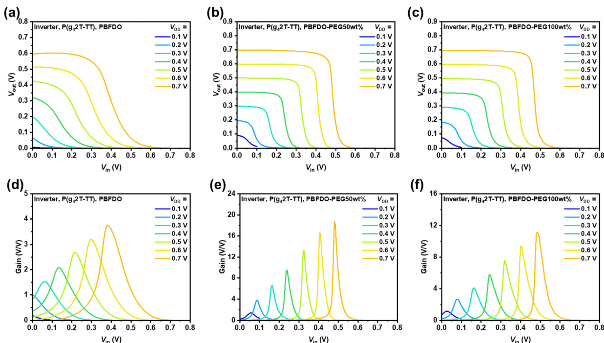
Fig. 6 OECTs-based complementary inverters. The voltage transfer characteristics and gain of inverters based on P( g_4 2T-TT) with different n-type channel materials (a) and (d) PBFD0, (b) and (e) PBFD0-PEG50wt%, (c) and (f) PBFD0-PEG100wt%.
