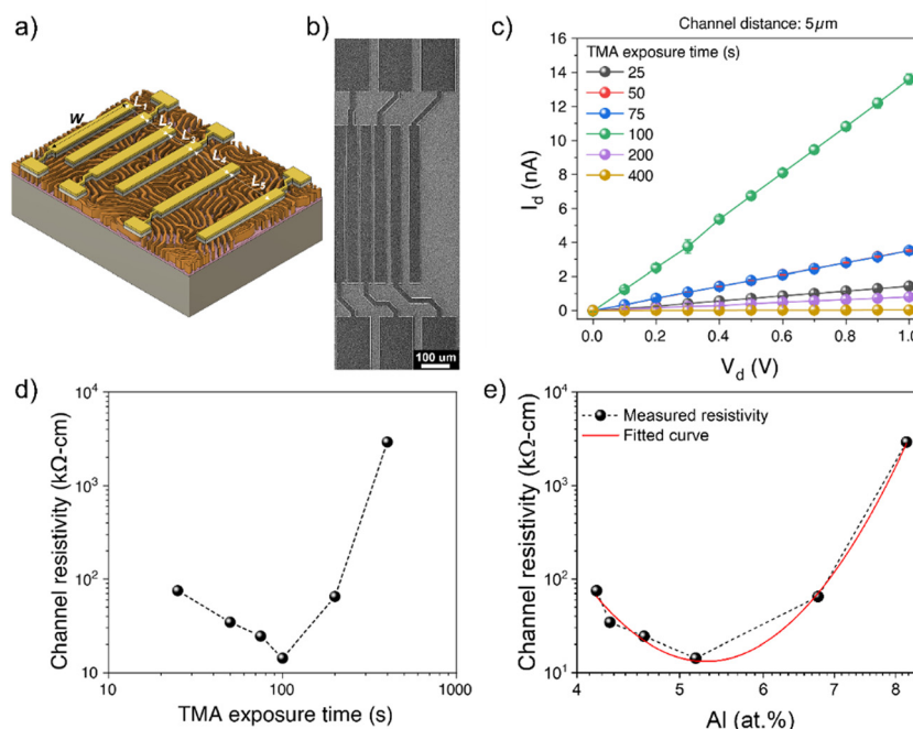
Fig. 4 (a) Schematic depiction of TLM electrodes onto AZO nanowires; contact spacing of electrodes are L_1 : 5 \mu\text{m} , L_2 : 8 \mu\text{m} , L_3 : 10 \mu\text{m} , L_4 : 15 \mu\text{m} , and L_5 25 \mu\text{m} . (b) Top-view SEM micrographs of the fabricated AZO nanostructured TLM devices. (c) Representative I - V plots of TLM devices with 5 \mu\text{m} of channel length of AZO nanowires with varying TMA exposure times (25, 50, 75, 100, 200, and 400 s). (d) Channel resistivity of AZO nanostructures with varying TMA exposure times, and (e) evolution of the channel resistivity of AZO nanostructures with varying Al atomic percentages.
