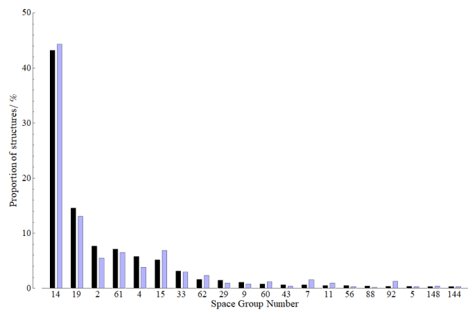
Fig. 3 The relative frequency of space groups observed for crystal structures (where Z' \leq 2 ) of molecules in the CSD with a molecular weight under 230 (black) and the subset of these molecules with no rotatable bonds selected for our CSP surveys. The distributions are presented for only the 20 most common space groups (of the general molecule case) for clarity.
