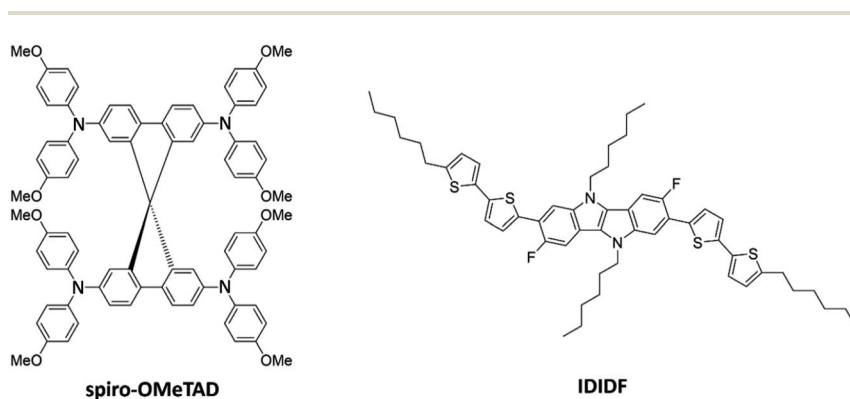
Fig. 1 Chemical structure of spiro-OMeTAD and the indolo[3,2- b ]indole-based IDIDF hole-transporting materials.
