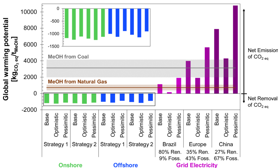
Fig. 13 Global warming potential (GWP), quantified as kg CO 2 ,eq per t MeOH , for DAC-PtM under all investigated wind-powered scenarios, compared against DAC-PtM driven with grid electricity (mix of energy sources) from Brazil, Europe, or China.
