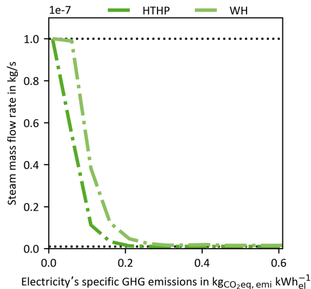
Fig. 9 Steam mass flow rate of the process leading to the maximal carbon removal rate CRR_{max} plotted over the electricity's greenhouse gas (GHG) emissions for a DACCS system for the waste heat (WH) and the high-temperature heat pump (HTHP) case.
