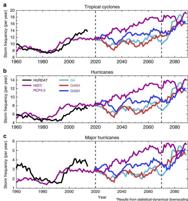
Fig. 13 Storm frequencies were modelled with a statistical dynamical downscaling method. (a) North Atlantic tropical cyclones (max wind-speed > 20 \text{ m s}^{-1} ), (b) hurricanes (max windspeed > 37 \text{ m s}^{-1} ), and (c) major hurricanes (max windspeed > 96 \text{ m s}^{-1} ) were simulated for both the SAI 2020–2070 period and the period after SAI was stopped abruptly (2070–2090). HURDAT is the historical observations of storm tracking for 1960–2014, while RCP4.5 represents the base case scenario. G4 is a global SAI scenario, whereas G4NH and G4SH are hemisphere-specific SAI scenarios. More simulation details and results are included in Table 1. Reprinted from Jones et al. , Nat. Commun. , 2017, 8, 1–10. Distributed under a Creative Commons Attribution 4.0 International License (CC BY 4.0) https://creativecommons.org/licenses/by/4.0/ .
