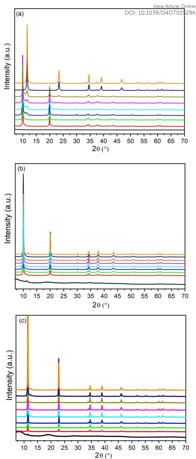
Fig. 2 XRPD of ZnAlCO 3 ( R =3) (a); ZAN/1 (b) and ZACI/1 (c) samples recovered at the increasing times (0 h, black ; 2 h, red line; 4 h, green line; 6 h, blue line; 20 h, cyan line; 24 h, pink line; 28 h, olive line; 48 h, navy line; 120 h, orange line). Reaction conditions: concentration of metal ions 0.5 M, y = 0.30, temperature: reflux.
