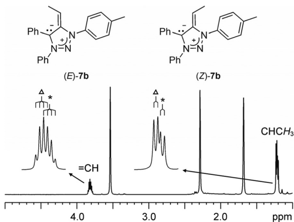
Fig. 4 The selected region of ^1\text{H} NMR ( \text{THF}-d_6 ) spectrum of in situ generated 7b . \Delta and * denote the major and minor isomers, respectively.
