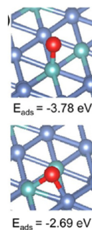
Fig. 10 Oxygen adsorption energy on NiMo(111) (Ni: blue, Mo: green, and O: red). Reproduced from ref. 125 with permission from American Chemical Society Catalysis, copyright 2021.
