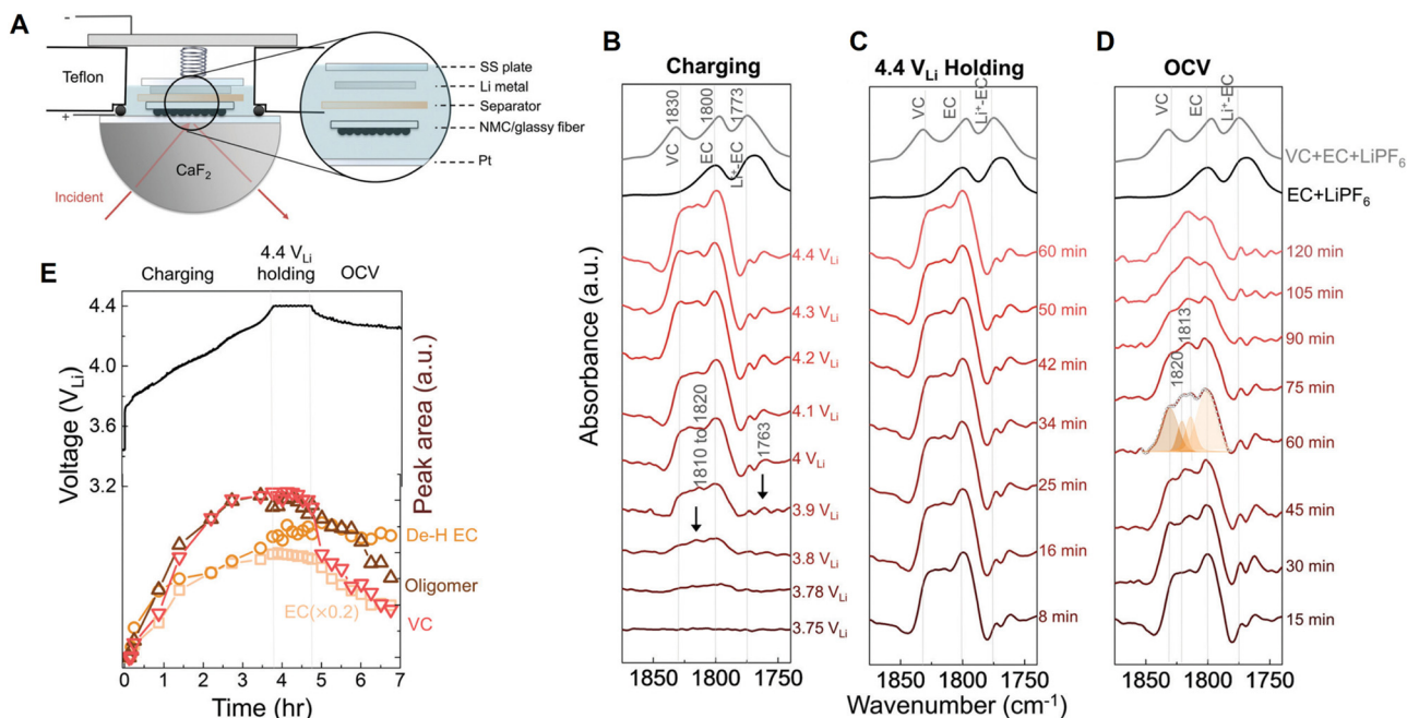
Fig. 14 (A) Schematic of an in situ FTIR cell. (B)–(D) In situ FTIR difference spectra on the \text{LiNi}_{0.8}\text{Co}_0.1\text{Mn}_{0.1}\text{O}_2 electrode during charging to 4.4 V (B), potentiostatic holding at 4.4 V (C), resting at OCV (D) in ethylene carbonate with 1.5 M \text{LiPF}_6 . (E) Corresponding electrochemical curve of the \text{LiNi}_{0.8}\text{Co}_0.1\text{Mn}_{0.1}\text{O}_2 electrode galvanostatically charged to 4.4 V, held at 4.4 V, and then rested at OCV; and deconvoluted IR intensity of peaks at 1800\text{ cm}^{-1} (ethylene carbonate), \sim 1813\text{ cm}^{-1} (dehydrogenated ethylene carbonate, De-H EC), \sim 1820\text{ cm}^{-1} (oligomers), and 1830\text{ cm}^{-1} (vinylene carbonate), respectively. OCV is an abbreviation for open circuit voltage, and the potential was referred to \text{Li}^+/\text{Li} . Reproduced with permission from ref. 159. Copyright 2020 the Royal Society of Chemistry.
