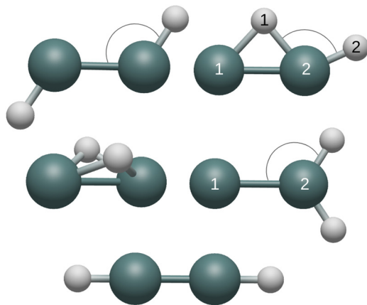
Fig. 1 From left to right and top to bottom, the five \text{Ge}_2\text{H}_2 structures of interest are shown: trans , monobridged, butterfly, germlydene, and linear. Structures containing non-equivalent atoms and bonds are henceforth referenced with the numbers in the figure. (ex: the terminal Ge–H bond of the monobridged structure would be \text{Ge}_{(2)}\text{--H}_{(2)} ).
