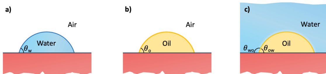
Fig. 2 Sessile droplets on a solid surface. (a) Water droplet in air, characterized by the water (w) contact angle \theta_w . (b) Oil droplet in air, characterized by the oil (o) contact angle \theta_o . (c) Oil droplet in water, characterized by the oil-in-water (o/w) contact angle \theta_{ow} . The latter is related to the water-in-oil (w/o) contact angle \theta_{wo} via the relation \theta_{wo} + \theta_{ow} = 180^\circ .
