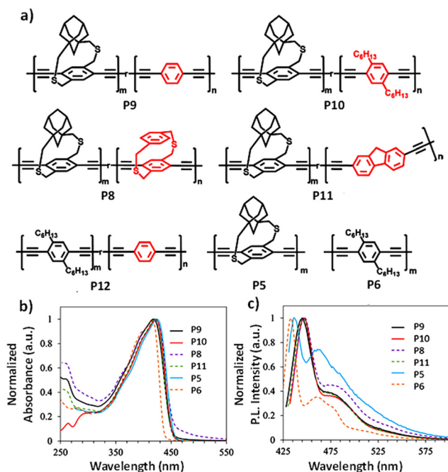
Fig. 18 (a) Chemical structures; (b) UV-vis absorption spectra and (c) emission spectra of P5 , P6 , and P8–P12 ( n \approx 20\% in the copolymers). Reproduced with permission from ref. 53. Copyright American Chemical Society (2023).
