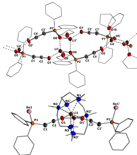
Fig. 4 Crystal structure of (top) 3a-Li and (bottom) 3c-Li (PMDETA). Ellipsoids are drawn at the 50% probability level. Important bond lengths [Å] and angles [°]: 3a-Li : P1–C1 1.677(4), C1–C2 1.230(6), C2–O1 1.216(5), P1–O1 1.510(3), P1–C1–C2 161.9(4), C1–C2–O1 176.7(5), P2–C3 1.673(4), C3–C4 1.231(6), C4–O2 1.206(5), P2–O6 1.509(3), P2–C3–C4 162.4(4), C1–C2–O1 176.7(5). 3c-Li (PMDETA): P1–Se1 2.132(1), P1–C1 1.698(6), C1–C2 1.243(8), C2–O1 1.222(7), O1–Li1 2.069(10), P1–C1–C2 147.8(5), C1–C2–O1 173.9(6).
