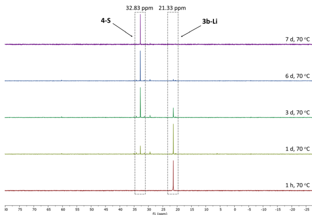
Fig. 3 Monitoring of the conversion of 3b-Li into 4-S by ^{31}\text{P}\{^1\text{H}\} NMR spectroscopy in THF- d_8 at 70 °C.
