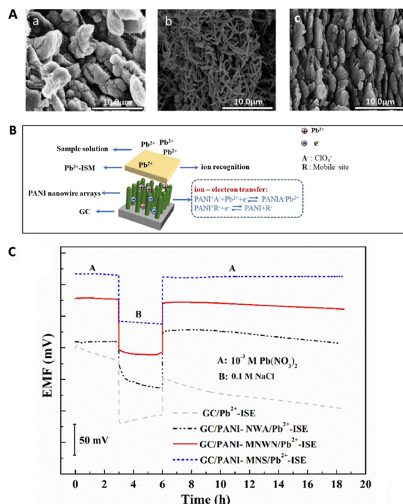
Fig. 6 (A) SEM images of PANI-NWA (a), PANI-MNWN (b), and PANI-MNS (c) deposited on a glassy carbon electrode by direct electrodeposition. (B) Sensing mechanism for a NWA-based ISE. (C) Potential curves of different \text{Pb}^{2+} -ISEs in 10^{-3} \text{ M Pb}(\text{NO}_3)_2 for 3 h, 0.1 \text{ M NaCl} for 3 h, and then 10^{-3} \text{ M Pb}(\text{NO}_3)_2 again for 12.5 h. 166 Copyright 2021, Elsevier.
