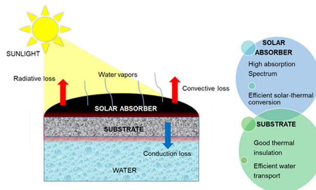
Fig. 1 Schematic illustration of solar-driven interfacial water evaporation.
