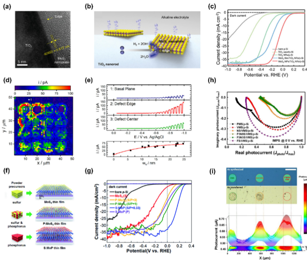
Fig. 2 (a) High-resolution TEM image of MoS 2 nanoplating having catalytically active edge sites decorated on TiO 2 nanorod. (b) Schematic illustration of MoS 2 nanoplating with large amounts of edges favorable for alkaline hydrogen evolution. (c) LSV curves of bare p-Si, TiO 2 seed/p-Si, TiO 2 nanorods/p-Si, MoS 2 film/TiO 2 nanorods/p-Si, and MoS 2 nanoplating/TiO 2 nanorods/p-Si photocathodes in 1 M KOH electrolyte. Copyright 2021, Wiley-VCH GmbH. (d) SECCM image with 1 \mu\text{m} resolution describing HER photocurrents of p-WSe 2 at -0.96 V vs. Ag/AgCl across the array of anodization defects. (e) I - V curves at basal plane, defect edge, and defect center in the SECCM image. Copyright 2020, American Chemical Society. (f) The photographic images of MoS 2 , phosphorus-doped MoS 2 , and sulfur-doped MoP thin film. (g) LSV curves of p-Si photocathodes with thin-film MoS 2 , P:MoS 2 , and S:MoS 2 catalysts. Copyright 2017, Royal Society of Chemistry. (h) IMPS Nyquist plot displaying the imaginary photocurrent vs. the normalized real photocurrent at 0 V vs. RHE. (i) Photocurrent mapping image of VMS, NS/VMS, and F1N9S/VMS catalysts. Copyright 2021, Elsevier.
