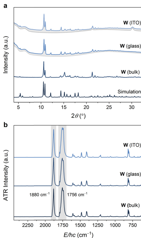
Fig. 3 (a) Powder X-ray diffractograms (Cu K\alpha , \lambda = 1.5406 \text{ \AA} ) of W coated on ITO and glass (blue traces, with grey traces representing uncoated substrate), compared with an experimental diffractogram of bulk W , as well as a simulated diffractogram. (b) ATR-FTIR spectra of W coated on ITO and glass, compared with the experimental spectrum collected on bulk W . See Fig. S13 and S17 (ESI†) for analogous Mo data.
