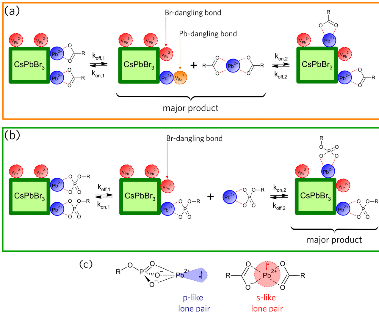
Fig. 3 Proposed mechanisms for the light-induced loss of surface components in hexane for (a) OA- and (b) OPA-capped \text{CsPbBr}_3 PNCs ( k_{\text{on}} : adsorption rate constant; k_{\text{off}} : desorption rate constant). (c) Molecular structures of components lost from the surface during light exposure, showing the hemidirected geometry and the p-like lone-pairs for \text{Pb}(\text{OPA}) , as well as the holodirected geometry and the s-like lone-pairs for \text{Pb}(\text{OA})_2 .
